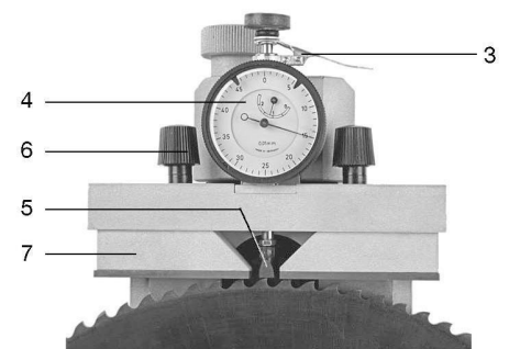
3 Indicator lever 4 Dial indicator 5 Measuring edge 6 Knurled nut 7 Support bars
